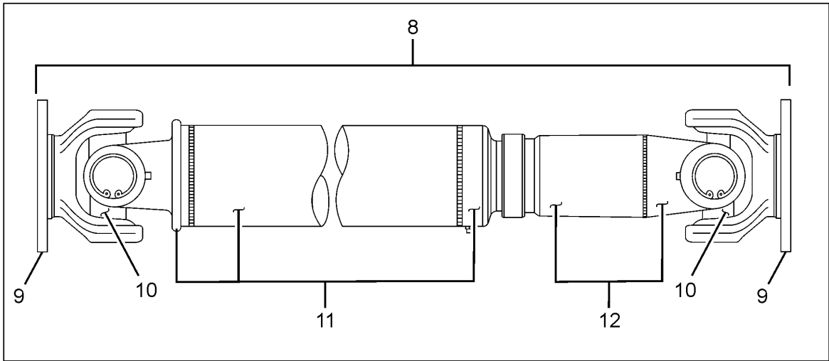
PROPELLER SHAFT REAR
